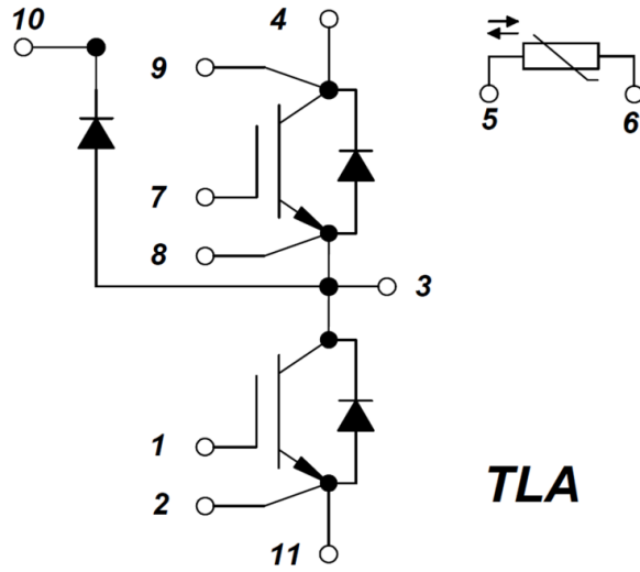
Figure 14. Circuit Diagram
