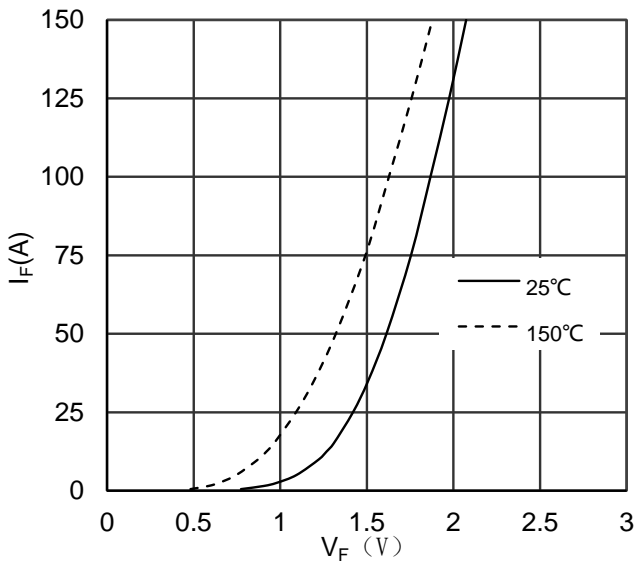
Figure 9. Diode Forward Characteristics Diode -inverter
