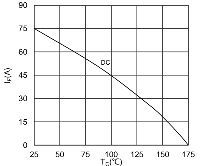
Figure 8. Forward current vs Case temperature Diode-inverter
