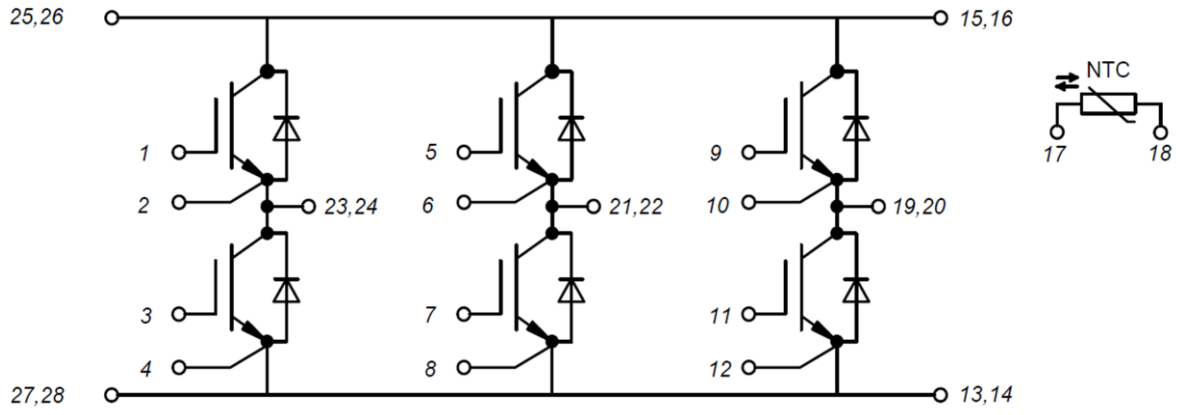
Figure 14. Circuit Diagram
