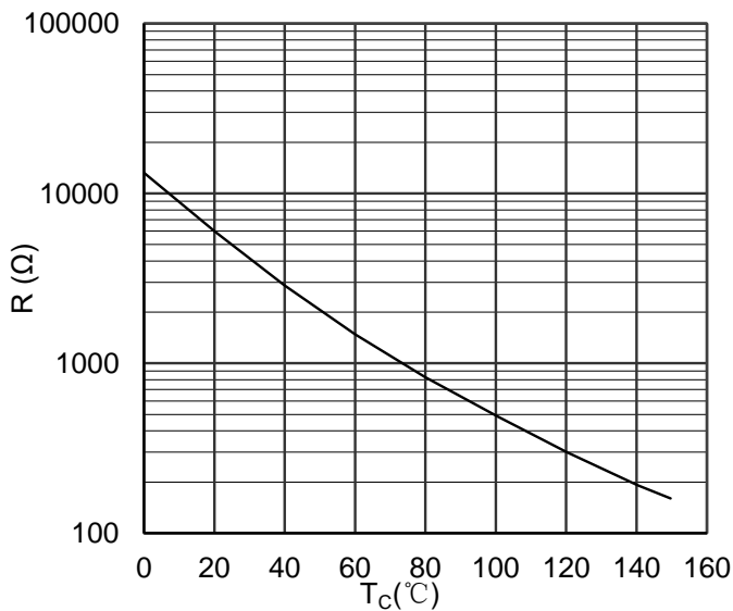
Figure 13. NTC Characteristics
