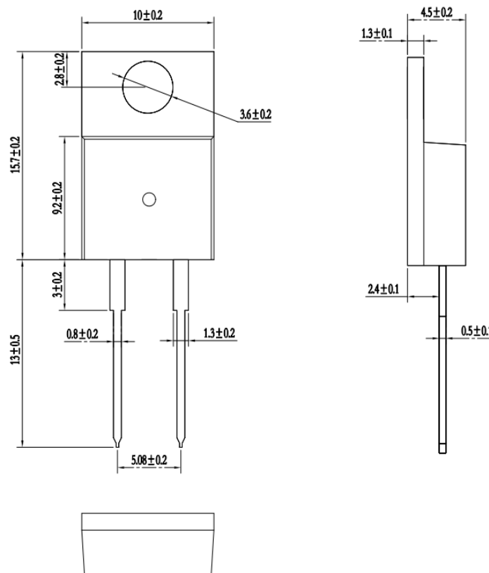
Figure 8. Package Outline
