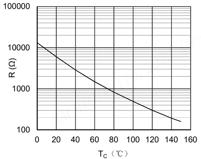
Figure 13. NTC Characteristics
