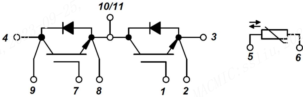
Figure 14. Circuit Diagram
